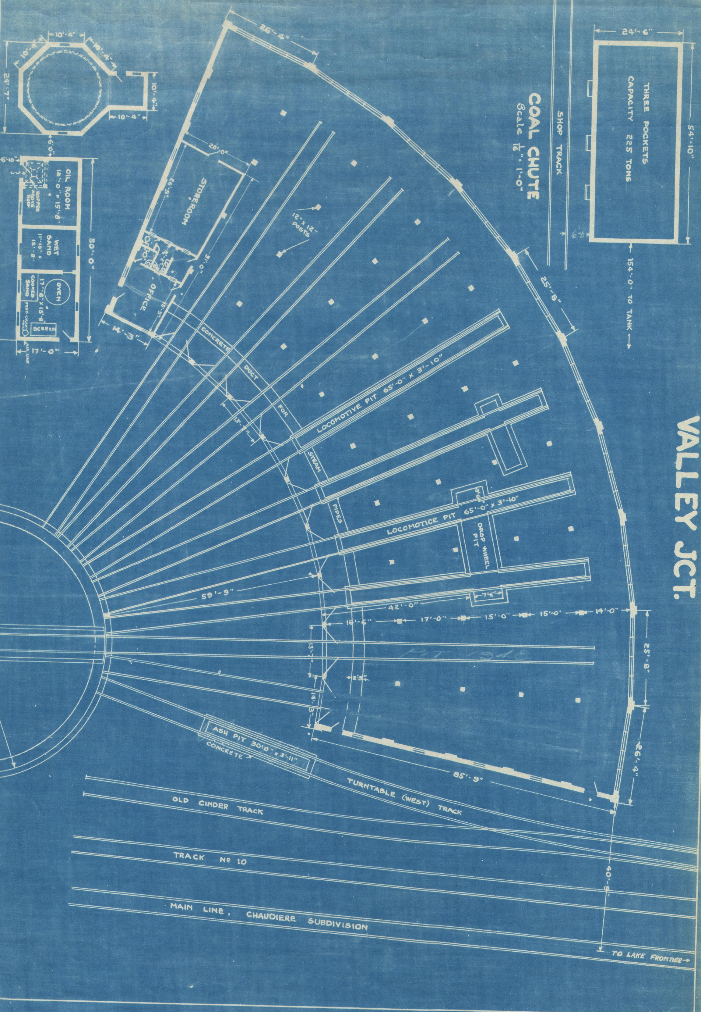
EAST WATER TANK Scale \frac{1}{16}'' = 1'-0''
